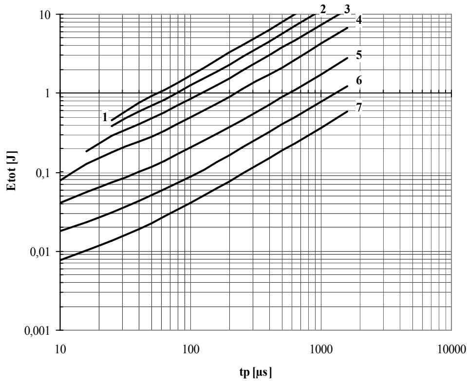
Fig. 25 Square wave loss energy per pulse
